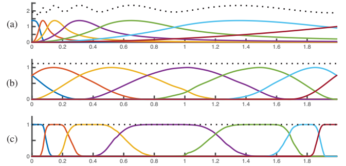
Fig. 12. Systems of spectral kernels of the (a) SGWT frame [10], (b) spectrum-adapted frame and (c) the signal-adapted frame, used for denoising.
