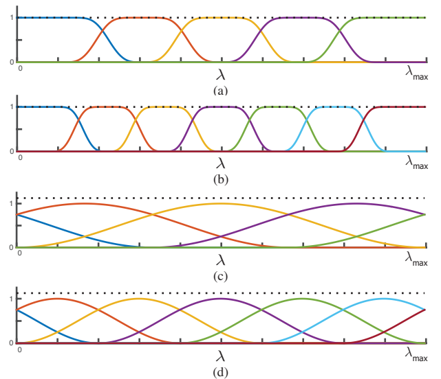
Fig. 2. UMT system of spectral kernels as given in Proposition 1 displayed for (a) J = 5 and (b) J = 7 spectral scales. The HCUT system of spectral kernels [24] displayed for (c) J = 5 and (d) J = 7 spectral scales.
