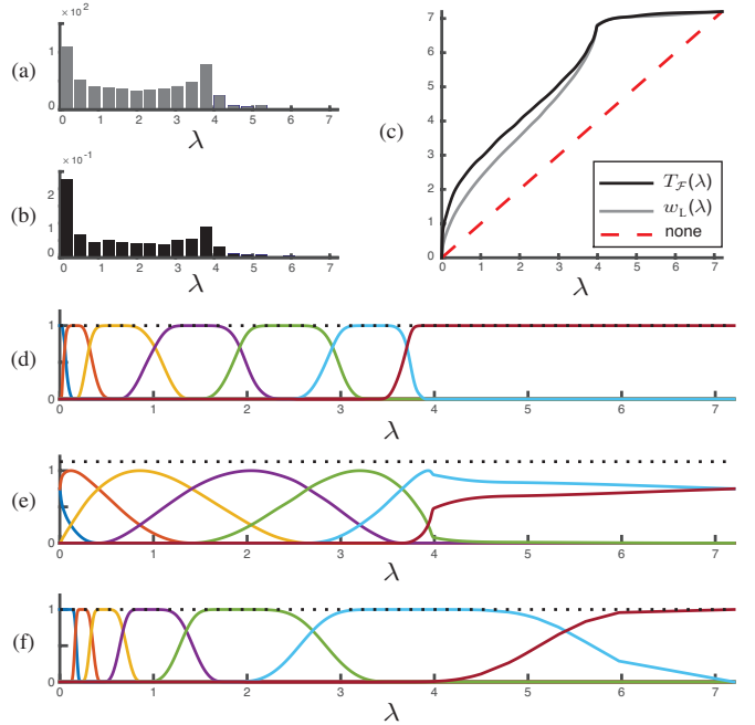
Fig. 6. (a) Histogram of the eigenvalues \Lambda_L(\mathcal{G}) of the Alameda graph. (b) Distribution of the ensemble energy spectral density \bar{e}_{\mathcal{F}} of the traffic dataset. (c) Constructed energy-equalizing transformation functions T_{\mathcal{F}}(\lambda) and the spectrum-adapting warping function w_L(\lambda) [24]. (d) Signal-adapted system of spectral kernels. (e) Spectrum-adapted system of spectral kernels [24]. (f) Meyer-like wavelet frame system of spectral kernels [11].
