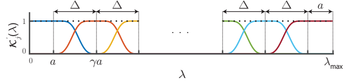
Fig. 1. Construction of UMT system of spectral kernels.
